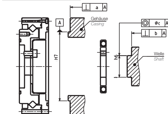
Montagetoleranzen Mounting Tolerance
