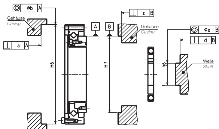
Montagetoleranzen Mounting Tolerance
