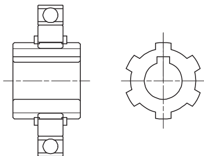
Spline (selbstzentrierend) Spline type (self-centering)
