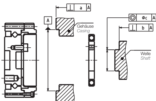
Montagetoleranzen Mounting Tolerance
